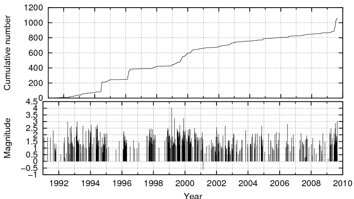
Figure 14. Cumulative number and magnitude of earthquakes in Eyjafjallajökull between 1991 and August 2009.
