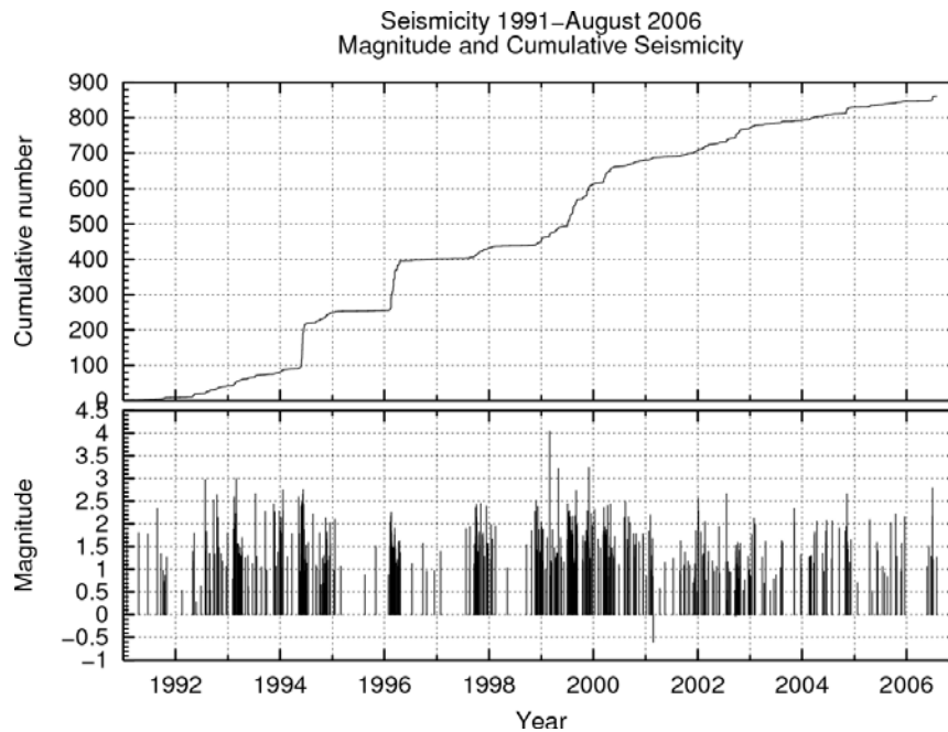
Figure 2. Upper: Cumulative number of earthquakes in and near to Eyjafjallajökull. Lower: Magnitude distribution (local moment magnitude scale, M_{lw} ).
